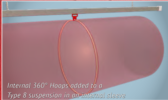
INTERNAL 360° HOOP
